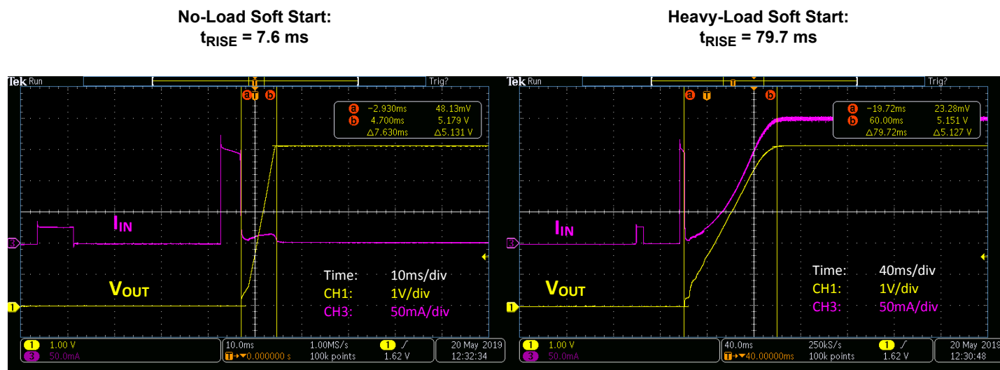
Figure 4.8. Si3404-Buck Non-Isolated EVB, 5 V, Class 2 Output Voltage Soft-Start at Low Load (Left) and Heavy Load (Right) Conditions
