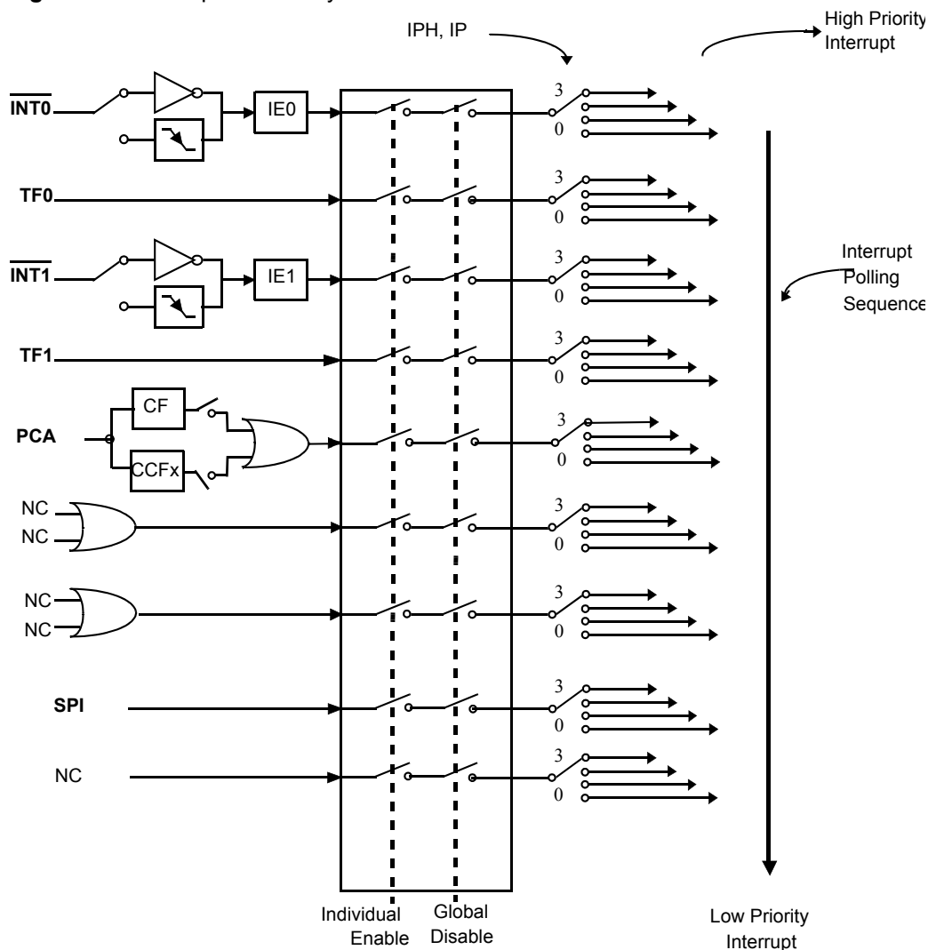
Figure 27. Interrupt Control System
