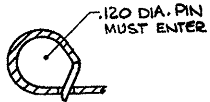
SECT. A-A
