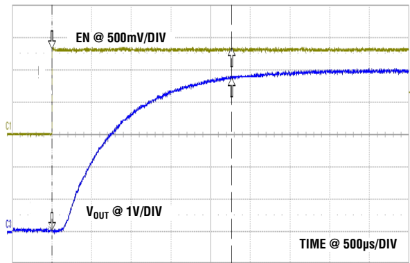
FIGURE 8. START-UP WAVEFORM
