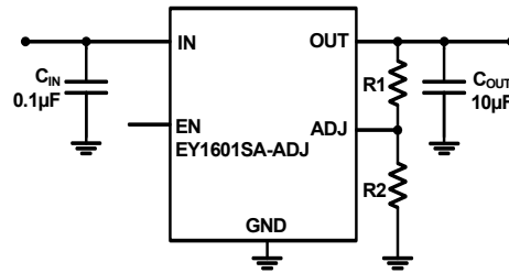
FIGURE 11. ADJUSTABLE VERSION
