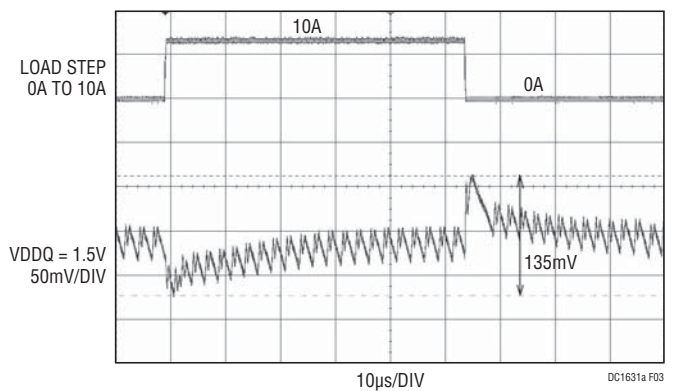
Figure 3. Load Step Response of the VDDQ on the DC1631A at V_{IN} = 12V . C_{OUT} = 2 \times \text{Sanyo 2R5TPE330M9} \parallel 1 \times 100\mu F \text{ X5R } 6.3V \text{ 1206} , L = 0.47\mu H , f_{SW} = 400kHz
