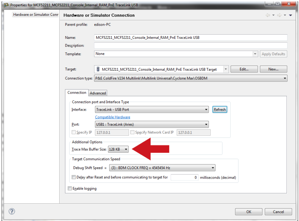
Figure 7-3: CodeWarrior: Set Trace Max Buffer Size
