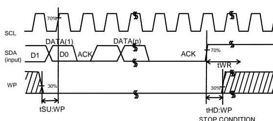
Figure 1-(d). WP Timing at Write Execution
