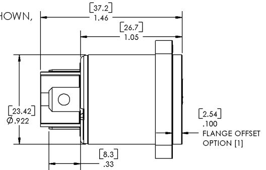
[F] TERMINALS
