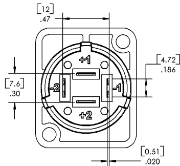
[F1] TERMINALS
