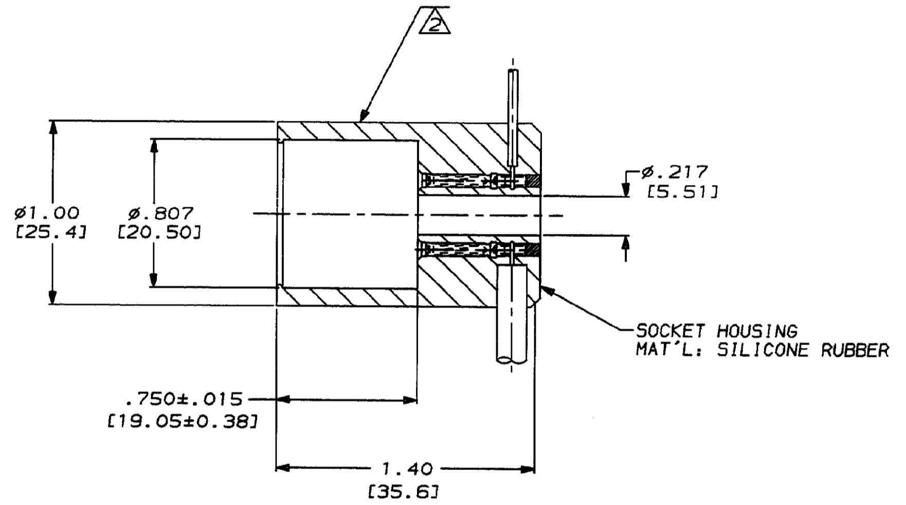
SECTION T-T
