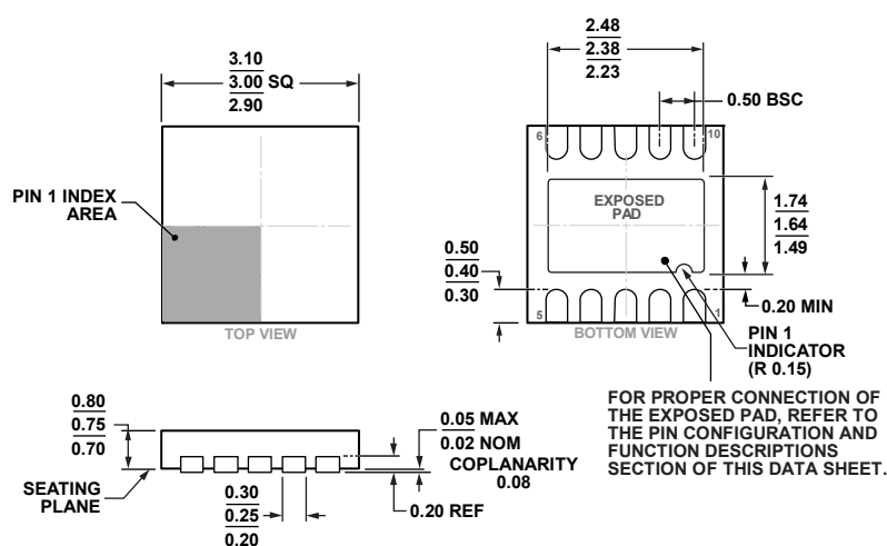
Figure 45. 10-Lead Lead Frame Chip Scale Package [LFCSP_WD] 3 mm × 3 mm, Very Very Thin, Dual Lead (CP-10-9) Dimensions shown in millimeters
