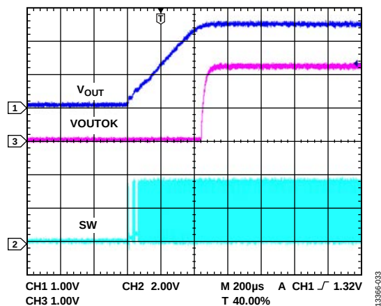
Figure 33. VOUTOK Function
