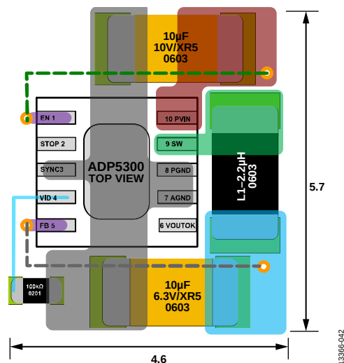
Figure 42. Typical PCB Layout
