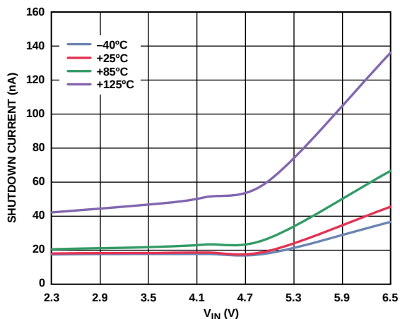
Figure 12. Shutdown Current vs. V_{IN} , EN = \text{Low}
