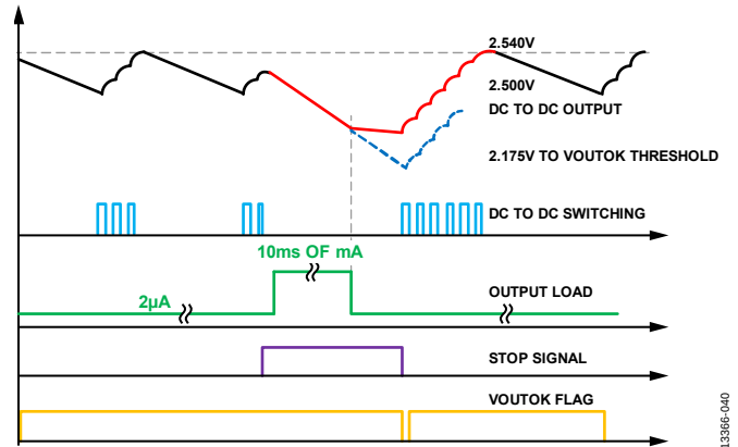
Figure 40. STOP Switching Operation Status
