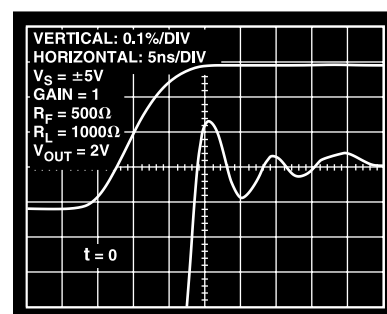
Figure 18. Settling Time
