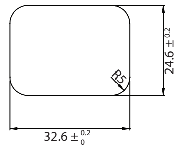
PANEL CUTOUT
