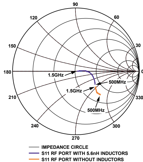
Figure 20. Input and Output Impedance Smith Chart (with Frequency Markers)
