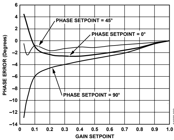
Figure 22. Phase Error vs. Gain Setpoint, 5V DC, 25°C, 880 MHz
