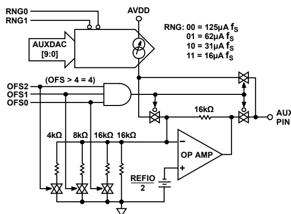
Figure 91. AUXDAC Simplified Circuit Diagram
