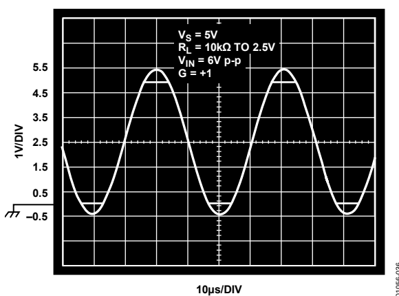
Figure 36. Output Voltage
