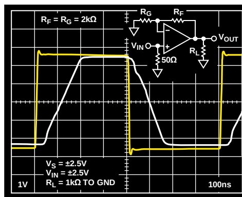
Figure 45. Overdrive Recovery
