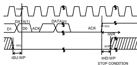
Figure 1-(d). WP Timing at Write Execution
