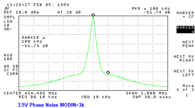
3.5V Phase Noise MODIN=3k
