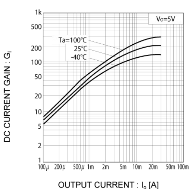
Fig.14 DC current gain vs. output current
