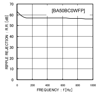
Fig.6 Ripple Rejection
