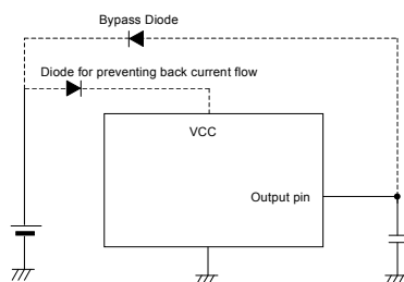
Fig.23 Bypass Diode
