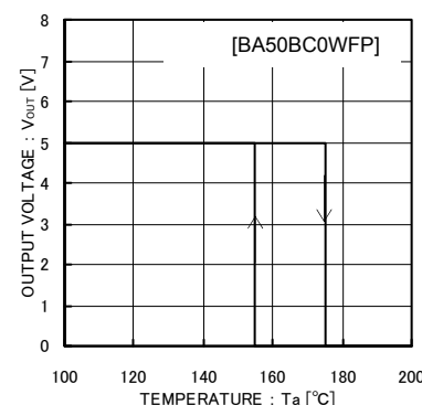
Fig.12 Thermal Shutdown Circuit
