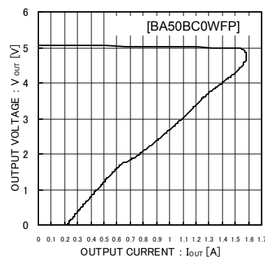
Fig.4 Load Stability
