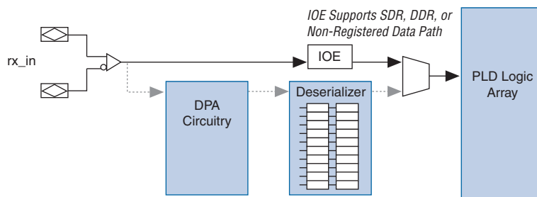
Figure 5-7. Deserializer Bypass
