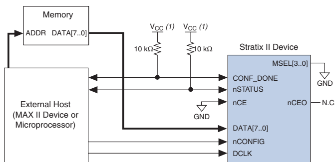
Figure 7–3. Single Device FPP Configuration Using an External Host
