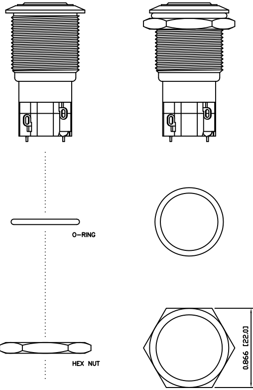
EXPLODED VIEW
