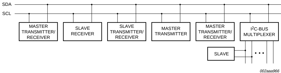
Fig 13. System configuration
