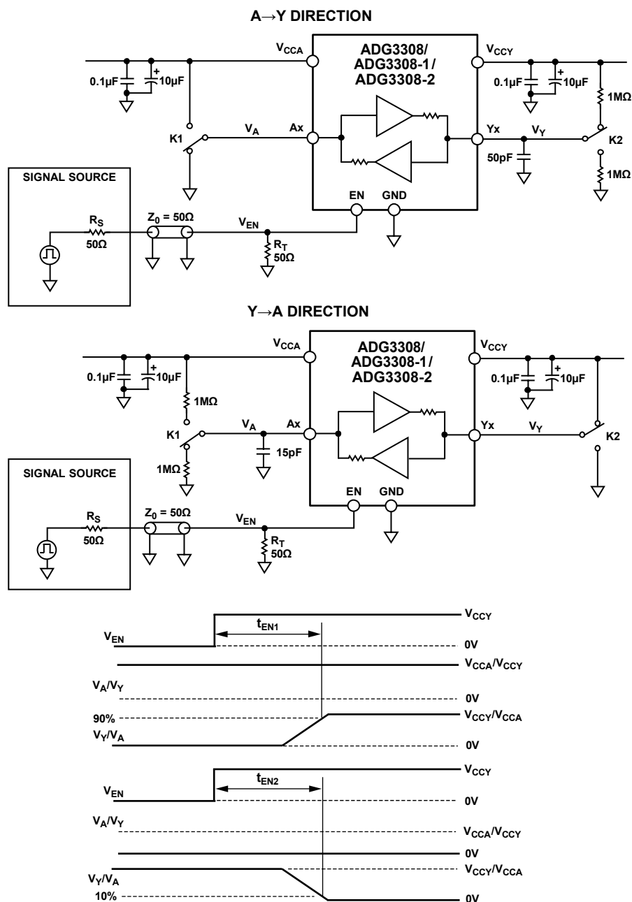
Figure 36. Enable Time
