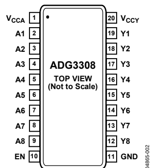
Figure 2. 20-Lead TSSOP
