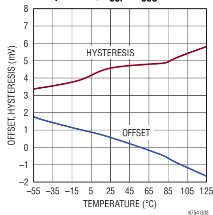
Input Offset and Hysteresis vs Temperature, V_{CCI} = V_{CCO} = 5.0V
