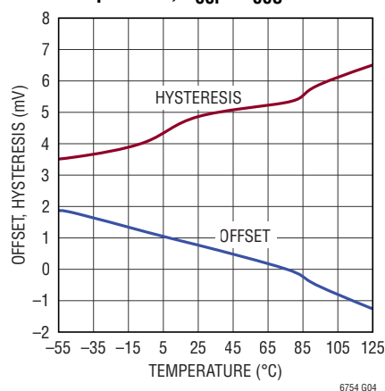
Input Offset and Hysteresis vs Temperature, V_{CCI} = V_{CCO} = 2.5V
