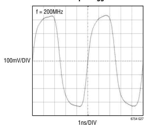
Differential Output Toggle Waveform
