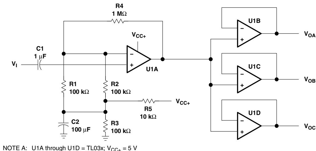
Figure 69. Audio-Distribution Amplifier Circuit
