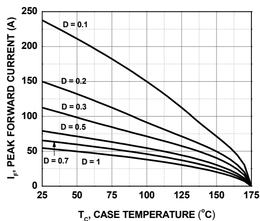
Figure 4. Current Derating
