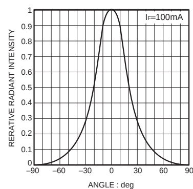
Fig.6 Radiant intensity
