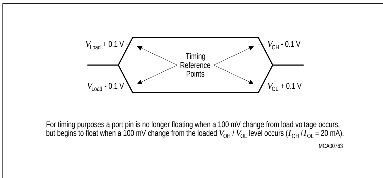
Figure 16 Float Waveforms
