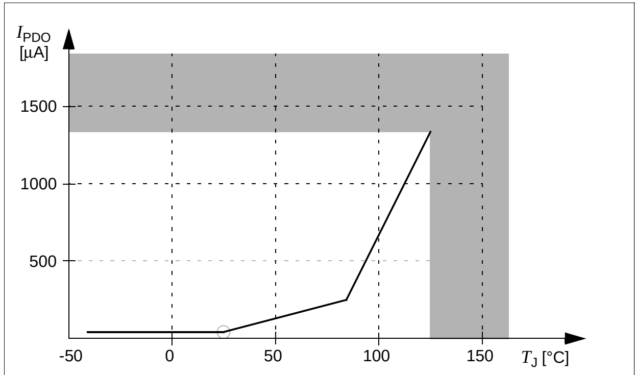
Figure 11 Sleep and Power Down Supply Current as a Function of Temperature
