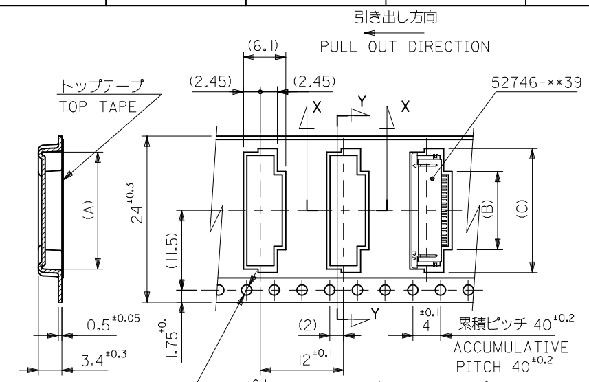
SECT.Y-Y
