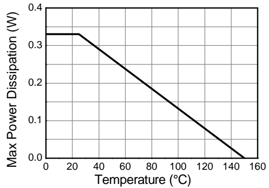
Derating Curve
