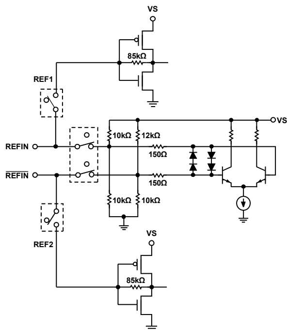
Figure 30. REF1N Equivalent Circuit for Non-XTAL Mode
