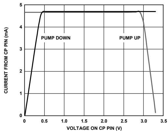
Figure 8. Charge Pump Characteristics @ V_{CP} = 3.3 V
