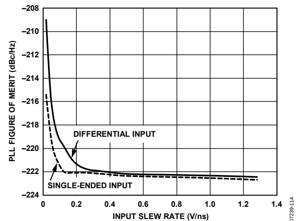
Figure 11. PLL Figure of Merit (FOM) vs. Slew Rate at \overline{REFIN}/REFIN
