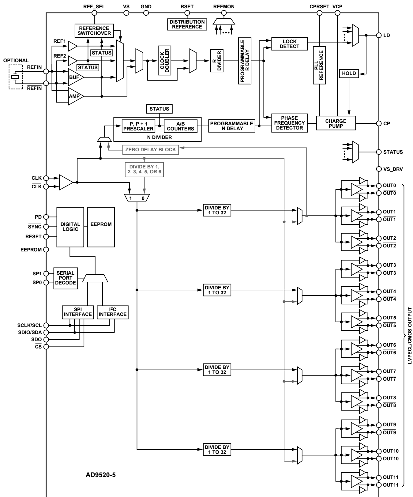
Figure 26. Clock Distribution or External VCO < 1600 MHz (Mode 1)
