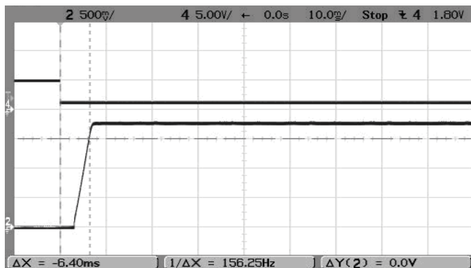
On/Off Enable Startup (Vin=5.5V, Vout=1.8V, Iout=5A, Cload=0) Trace 4=Enable, Trace2=Vout
