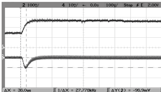
Step Load Transient Response (Vin=5V, Vout=1.5V, Cload=0, Iout=2.5A to 5A) Trace 2=Vout, 100 mV/div. Trace 4=Iout, 2A/div.
