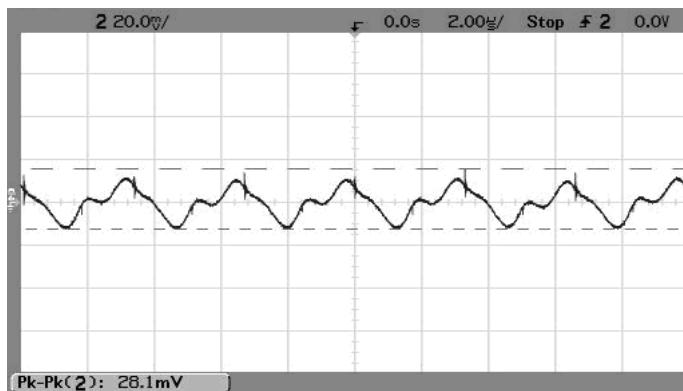
Output Ripple and Noise (Vin=5V, Vout=2.5V, Iout=5A, Cload=0, ScopeBW=100MHz)
