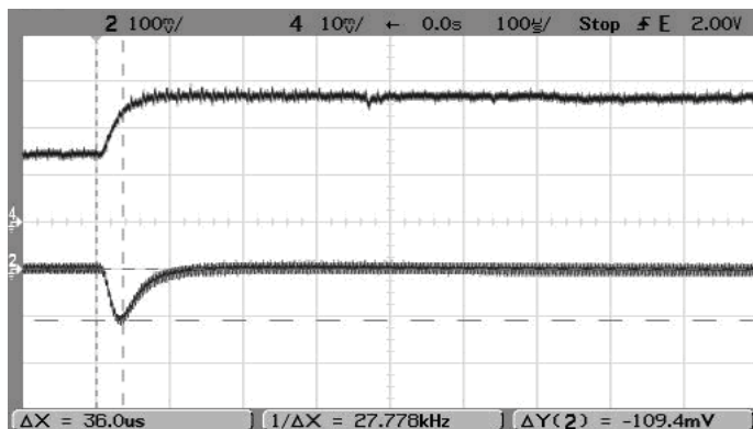
Step Load Transient Response (Vin=5V, Vout=2.5V, Cload=0, Iout=2.5A to 5A) Trace 2=Vout, 100 mV/div. Trace 4=Iout, 2A/div.
