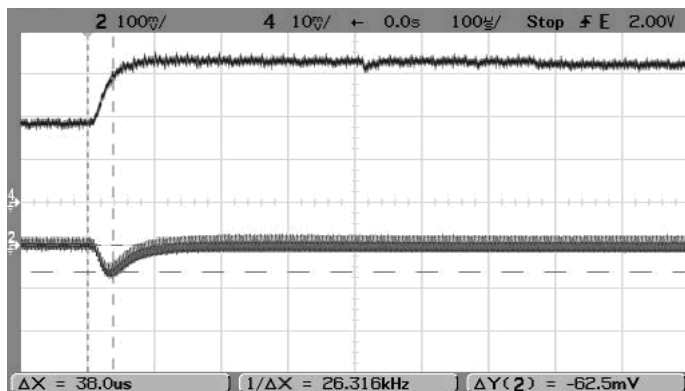
Step Load Transient Response (Vin=5V, Vout=1.5V, Cload=0, Iout=1.5A to 3A) Trace 2=Vout, 100 mV/div. Trace 4=Iout, 1A/div.
