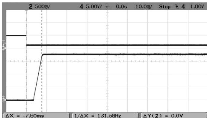
On/Off Enable Startup (Vin=5.5V, Vout=1.8V, Iout=3A, Cloud=0) Trace 4=Enable, Trace 2=Vout
