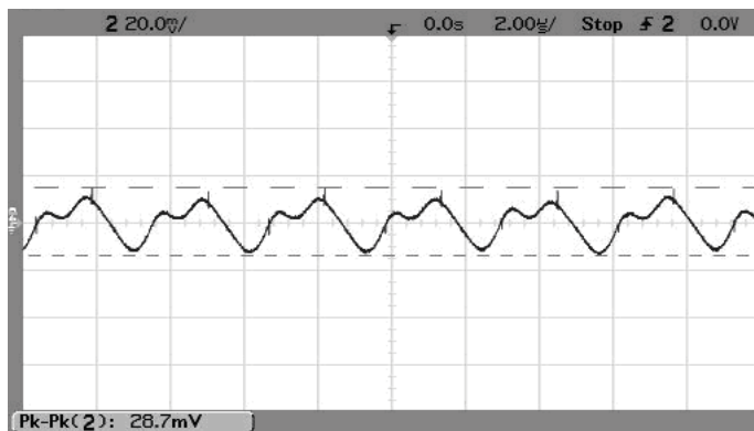
Output Ripple and Noise (Vin=5V, Vout=2.5V, Iout=3A, Cload=0, ScopeBW=100MHz)
