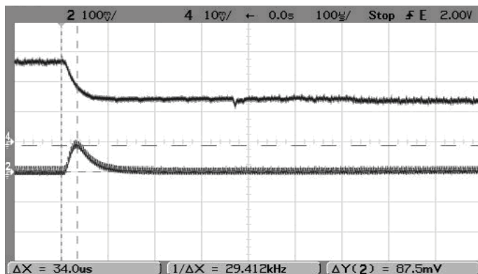
Step Load Transient Response (Vin=5V, Vout=1.8V, Cload=0, Iout=5A to 2.5A) Trace 2=Vout, 100 mV/div. Trace 4=Iout, 2A/div.
