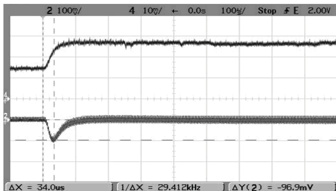
Step Load Transient Response (Vin=5V, Vout=1.2V, Cload=0, Iout=2.5A to 5A) Trace 2=Vout, 100 mV/div. Trace 4=Iout, 2A/div.
