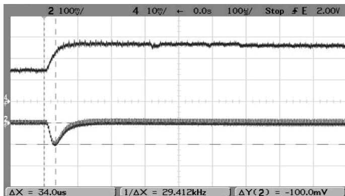
Step Load Transient Response (Vin=5V, Vout=1.8V, Cload=0, Iout=2.5A to 5A) Trace 2=Vout, 100 mV/div. Trace 4=Iout, 2A/div.
