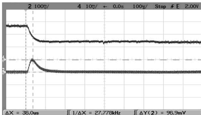
Step Load Transient Response (Vin=5V, Vout=2.5V, Cload=0, Iout=5A to 2.5A) Trace 2=Vout, 100 mV/div. Trace 4=Iout, 2A/div.
