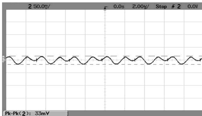
Output Ripple and Noise (Vin=5V, Vout=3.3V, Iout=5A, Cload=0, ScopeBW=100MHz)
