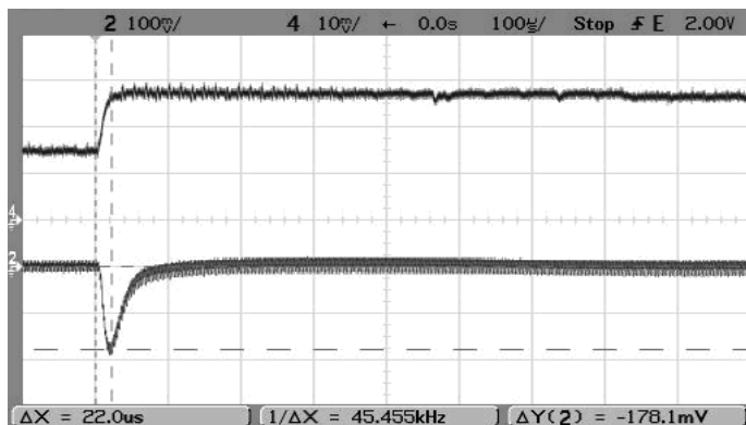
Step Load Transient Response (Vin=5V, Vout=3.3V, Cload=0, Iout=2.5A to 5A) Trace 2=Vout, 100 mV/div. Trace 4=Iout, 2A/div.
