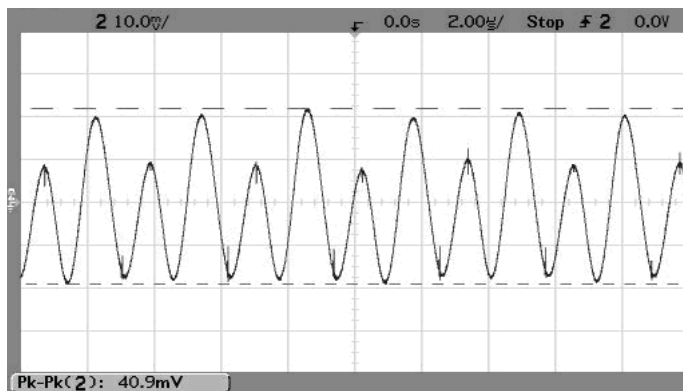
Output Ripple and Noise (Vin=5V, Vout=1.2V, Iout=3A, Cload=0, ScopeBW=100MHz)
