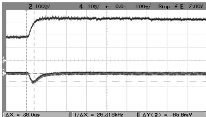
Step Load Transient Response (Vin=5V, Vout=2.5V, Cload=0, Iout=1.5A to 3A) Trace 2=Vout, 100 mV/div. Trace 4=Iout, 1A/div.
