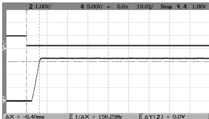
On/Off Enable Startup (Vin=5.5V, Vout=3.3V, Iout=5A, Cload=0) Trace 4=Enable, Trace2=Vout
