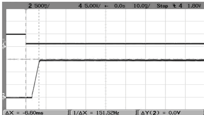
On/Off Enable Startup (Vin=5.5V, Vout=1.5V, Iout=5A, Cload=0) Trace 4=Enable, Trace2=Vout
