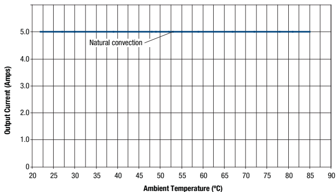
OKY-T/5-W5 Maximum Current Temperature Derating at Sea Level (VIN = 3.3 to 5V, Vout = 0.75 to 3.3V, VIN > Vout + 0.5V)
