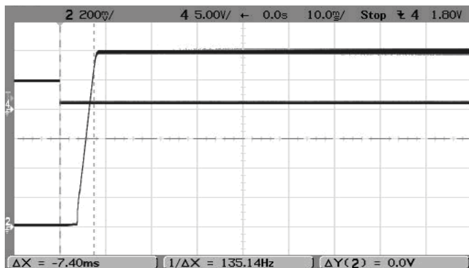
On/Off Enable Startup (Vin=5.5V, Vout=1.2V, Iout=3A, Cload=0) Trace 4=Enable, Trace 2=Vout
