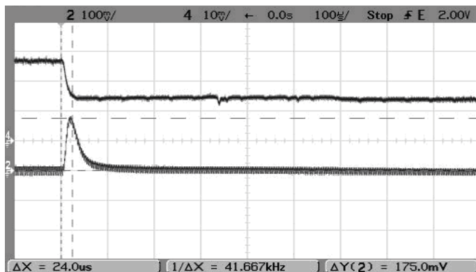
Step Load Transient Response (Vin=5V, Vout=3.3V, Cload=0, Iout=5A to 2.5A) Trace 2=Vout, 100 mV/div. Trace 4=Iout, 2A/div.
