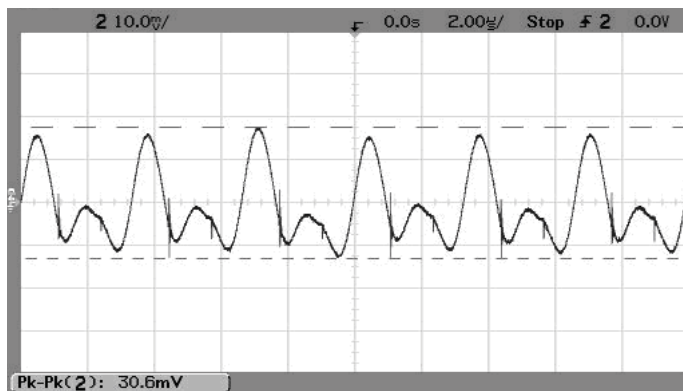
Output Ripple and Noise (Vin=5V, Vout=1.8V, Iout=5A, Cload=0, ScopeBW=100MHz)
