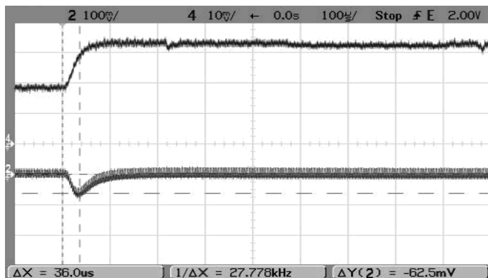
Step Load Transient Response (Vin=5V, Vout=1.8V, Cloud=0, Iout=1.5A to 3A) Trace 2=Vout, 100 mV/div. Trace 4=Iout, 1A/div.
