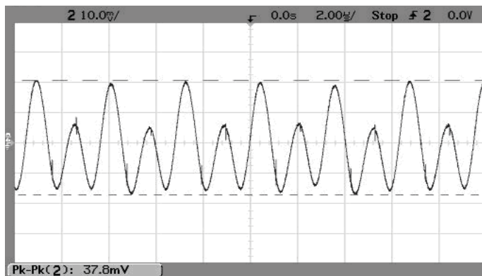
Output Ripple and Noise (Vin=5V, Vout=1.5V, Iout=3A, Cload=0, ScopeBW=100MHz)
