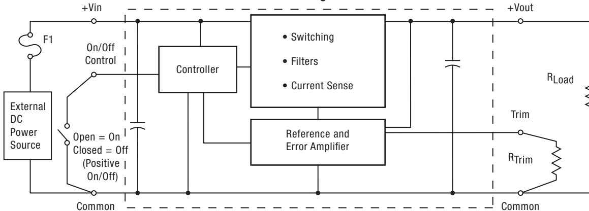
Figure 1. OKY-T/3, -T/5
