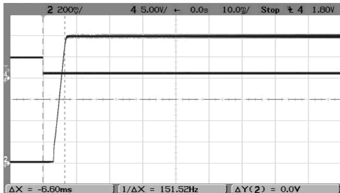
On/Off Enable Startup (Vin=5.5V, Vout=1.2V, Iout=5A, Cload=0) Trace 4=Enable, Trace2=Vout
