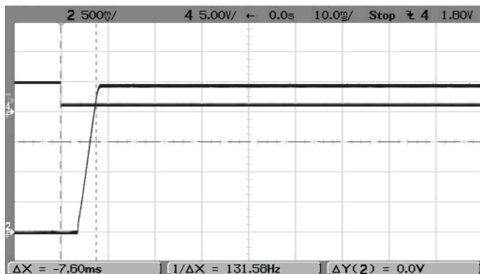
On/Off Enable Startup (Vin=5.5V, Vout=2.5V, Iout=3A, Cload=0) Trace 4=Enable, Trace 2=Vout
