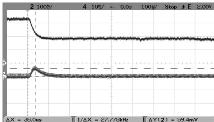
Step Load Transient Response (Vin=5V, Vout=1.8V, Cloud=0, Iout=3A to 1.5A) Trace 2=Vout, 100 mV/div. Trace 4=Iout, 1A/div.
