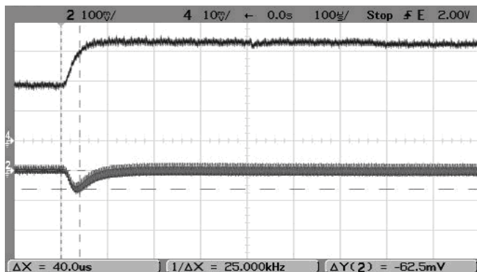
Step Load Transient Response (Vin=5V, Vout=1.2V, Cload=0, Iout=1.5A to 3A) Trace 2=Vout, 100 mV/div. Trace 4=Iout, 1A/div.
