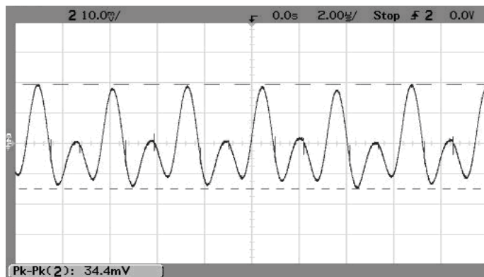
Output Ripple and Noise (Vin=5V, Vout=1.8V, Iout=3A, Cloud=0, ScopeBW=100MHz)
