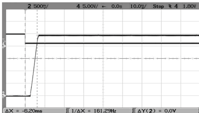
On/Off Enable Startup (Vin=5.5V, Vout=2.5V, Iout=5A, Cload=0) Trace 4=Enable, Trace2=Vout
