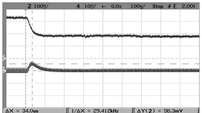
Step Load Transient Response (Vin=5V, Vout=1.2V, Cload=0, Iout=3A to 1.5A) Trace 2=Vout, 100 mV/div. Trace 4=Iout, 1A/div.
