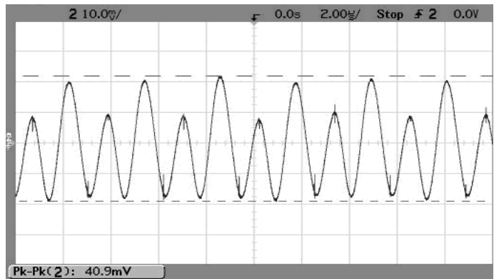
Output Ripple and Noise (Vin=5V, Vout=1.2V, Iout=3A, Cload=0, ScopeBW=100MHz)
