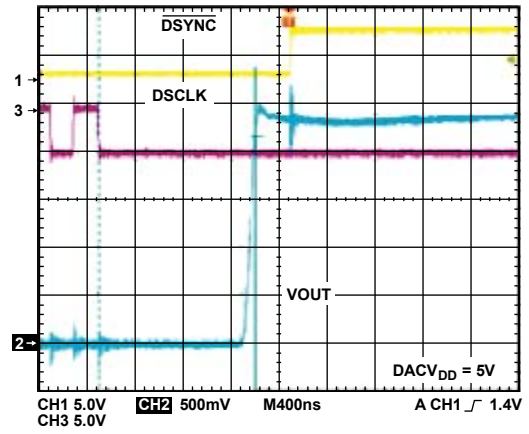
Figure 16. DAC Exiting Power-Down to Midscale
