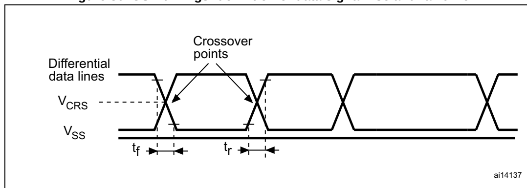
Figure 30. USB timings: definition of data signal rise and fall time
