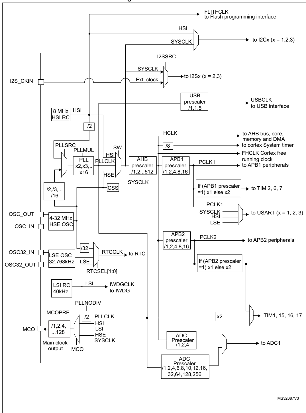
Figure 2. Clock tree
