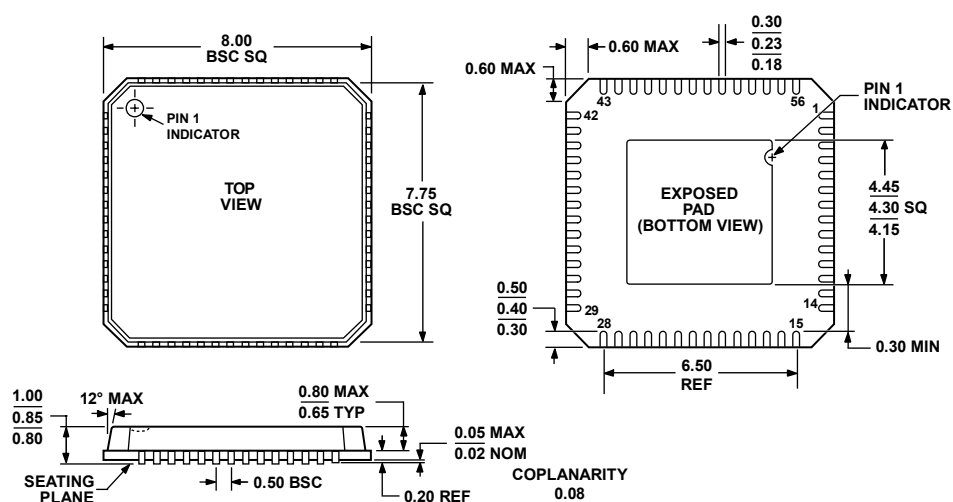
Figure 49. 56-Lead Lead Frame Chip Scale Package [LFCSP_VQ] 8 mm x 8 mm Body, Very Thin Quad (CP-56-2) Dimensions shown in millimeters
