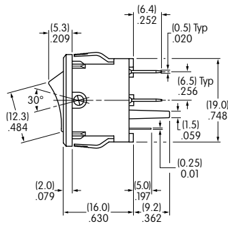
Single Pole
