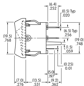
Single Pole
