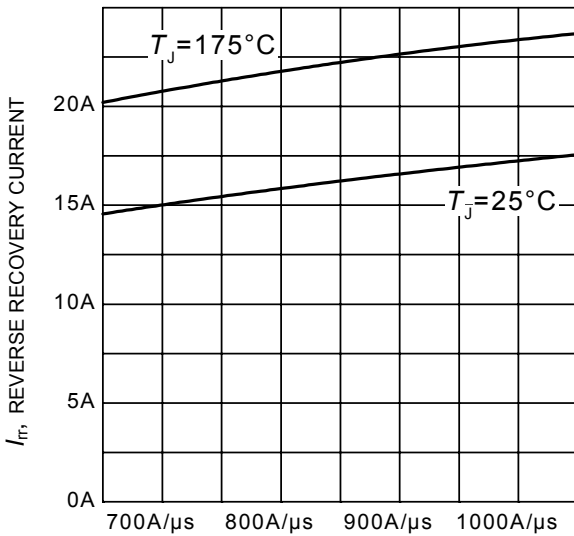
di_F/dt , DIODE CURRENT SLOPE Figure 25. Typical reverse recovery current as a function of diode current slope
