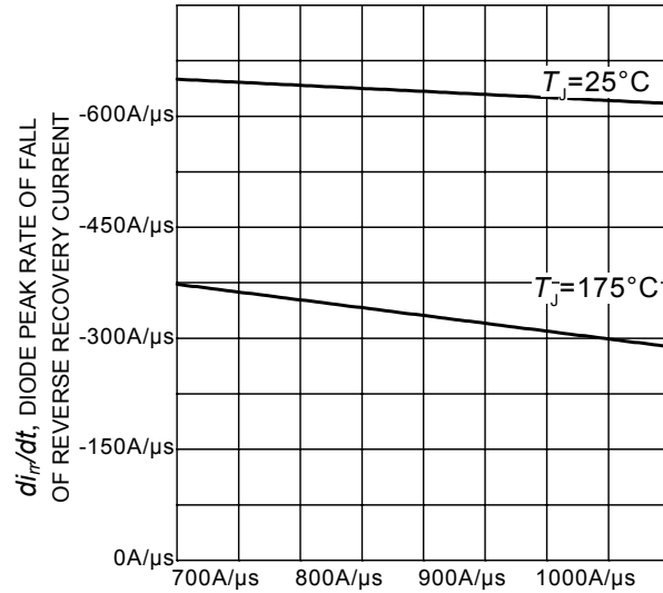
di_F/dt , DIODE CURRENT SLOPE Figure 26. Typical diode peak rate of fall of reverse recovery current as a function of diode current slope
