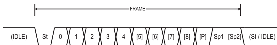
Figure 14-4. Frame Formats
