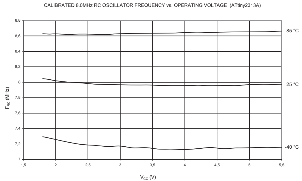
Figure 23-46. Calibrated 8 MHz RC Oscillator Frequency vs. V_{CC}
