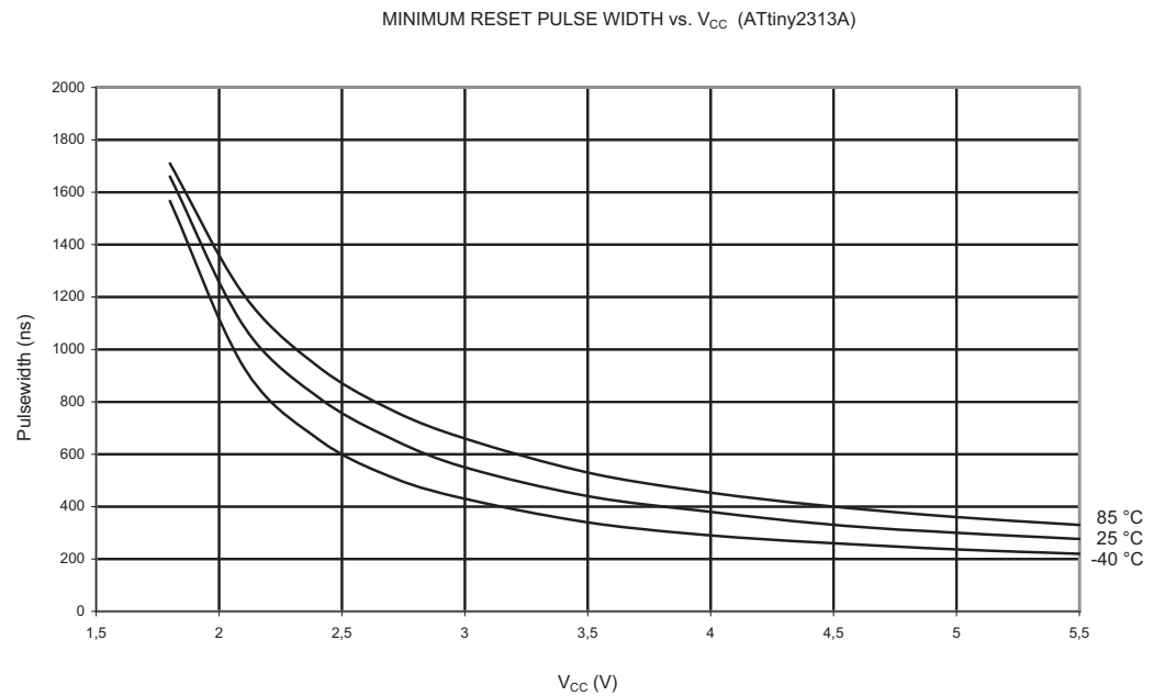
Figure 23-45. Minimum Reset Pulse Width vs. V_{CC}
