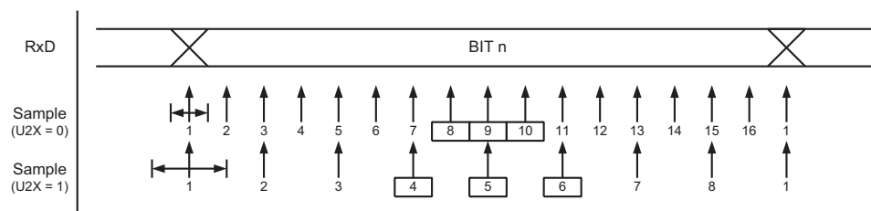
Figure 14-6. Sampling of Data and Parity Bit
