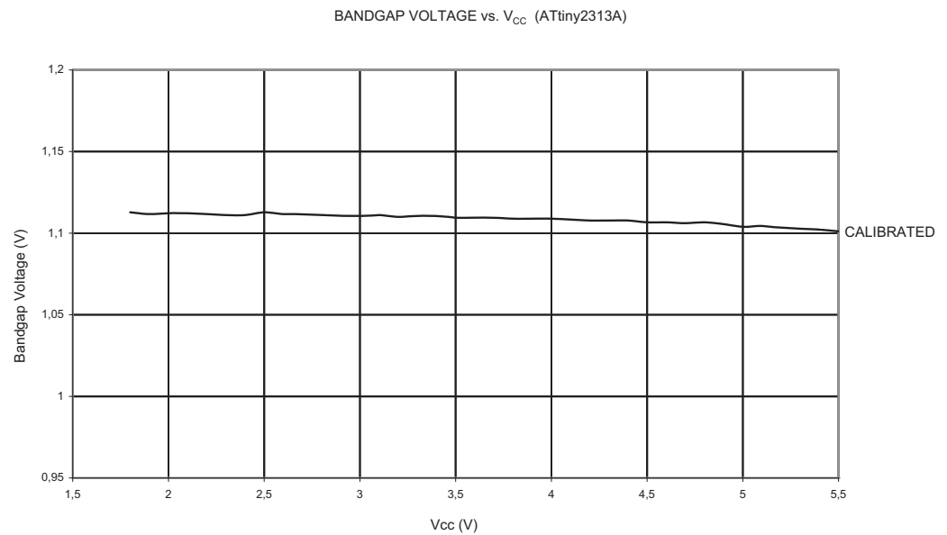
Figure 23-40. Bandgap Voltage vs. Supply Voltage
