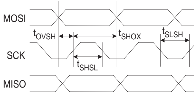
Figure 22-6. Serial Programming Timing
