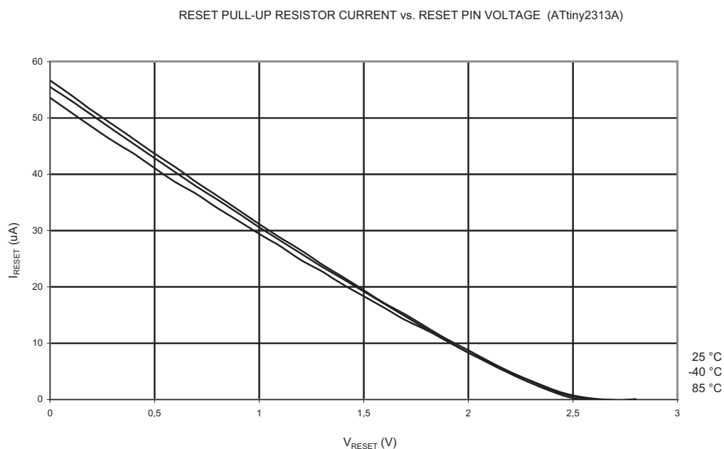
Figure 23-21. Reset Pull-up Resistor Current vs. Reset Pin Voltage ( V_{CC} = 2.7V )
