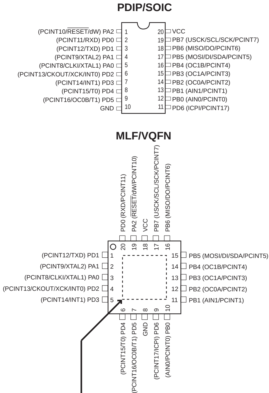
Figure 1-1. Pinout ATtiny2313A/4313
