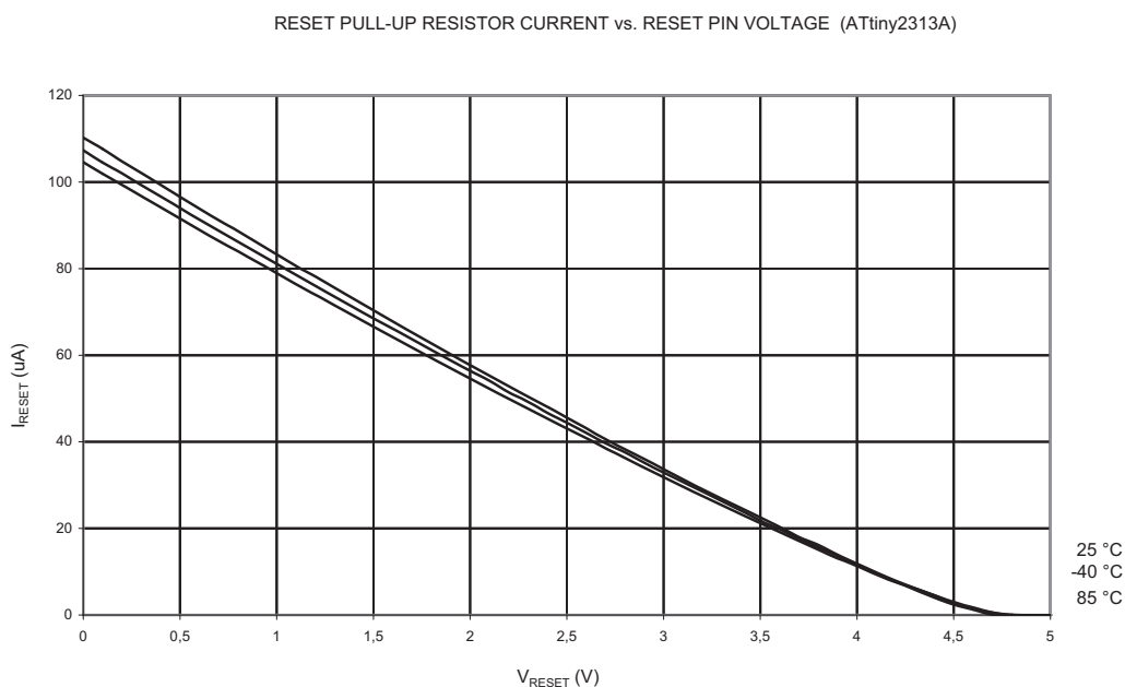
Figure 23-22. Reset Pull-up Resistor Current vs. Reset Pin Voltage ( V_{CC} = 5V )
