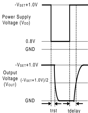
Figure 11. CMOS Output
