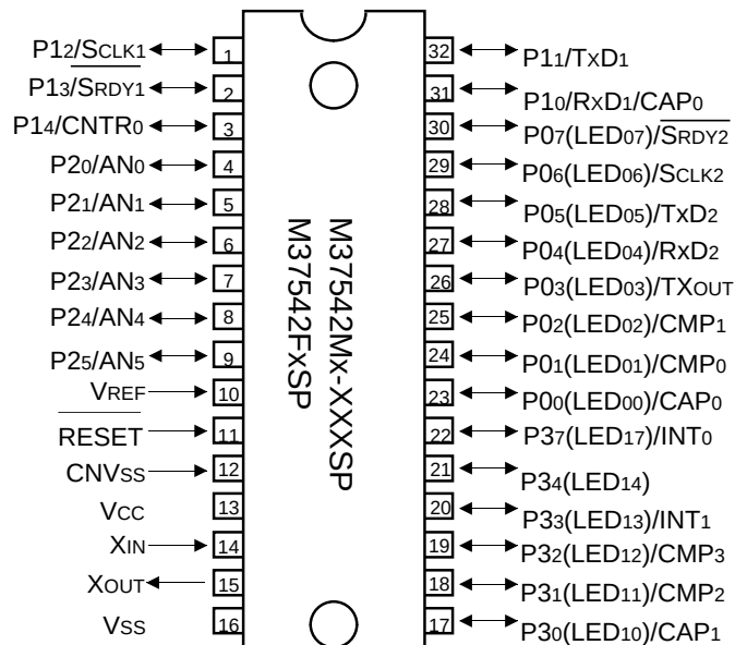
Package type: PRDP0032BA-A (32P4B)
