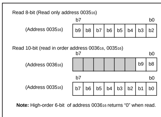
Fig. 69 Structure of A/D conversion register
