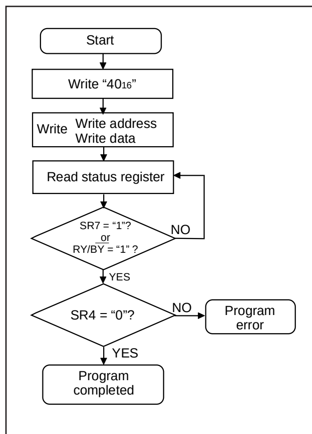
Fig. 102 Program flowchart
