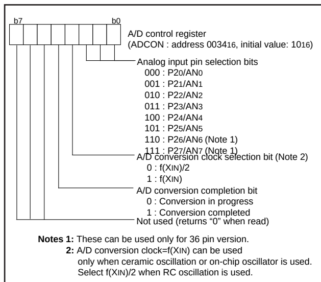
Fig. 68 Structure of A/D control register
