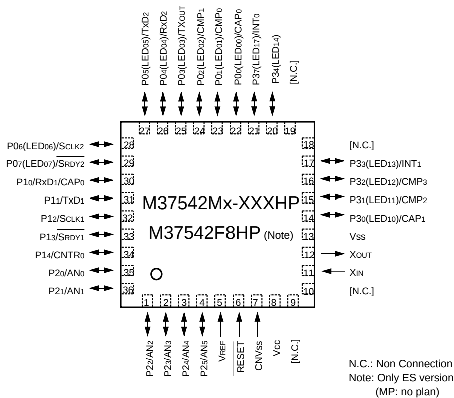
Package type: PWQN0036KA-A (36PJW-A)
