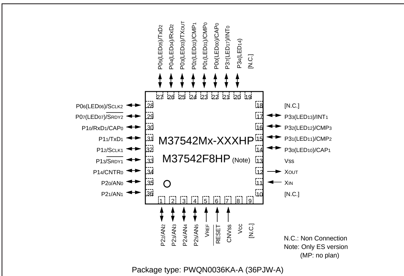
Fig. 4 Pin configuration (Package type: PWQN0036KA-A)
