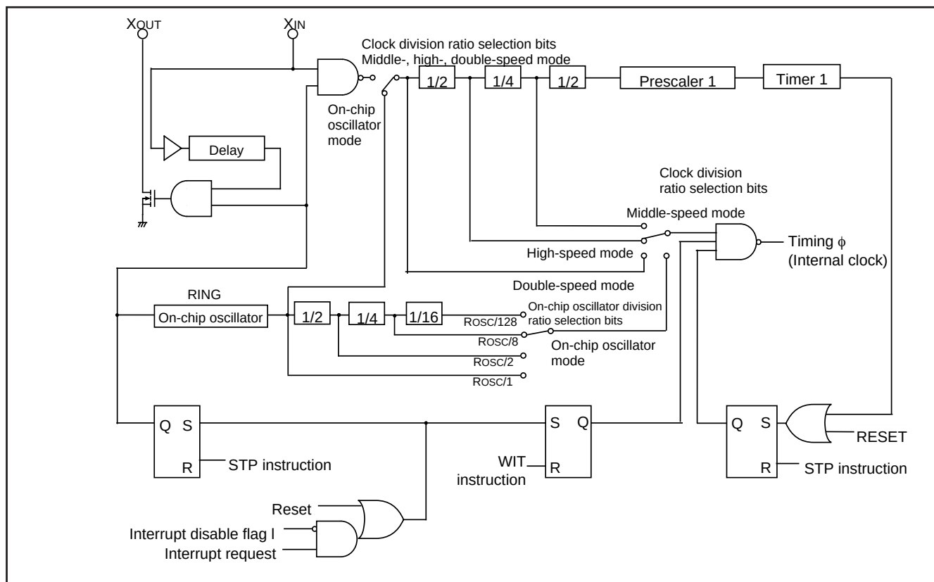
Fig. 83 Block diagram of internal clock generating circuit (for RC oscillation)
