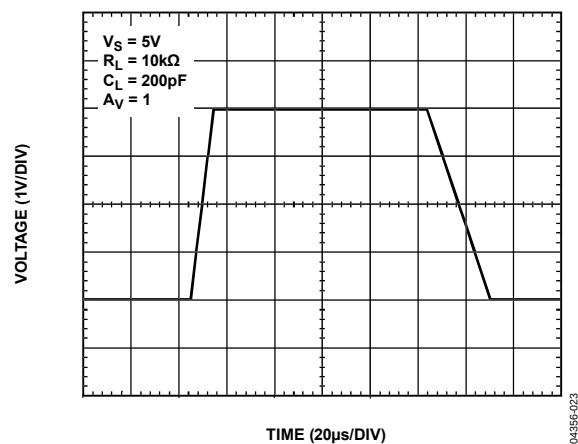
Figure 23. Large Signal Transient
