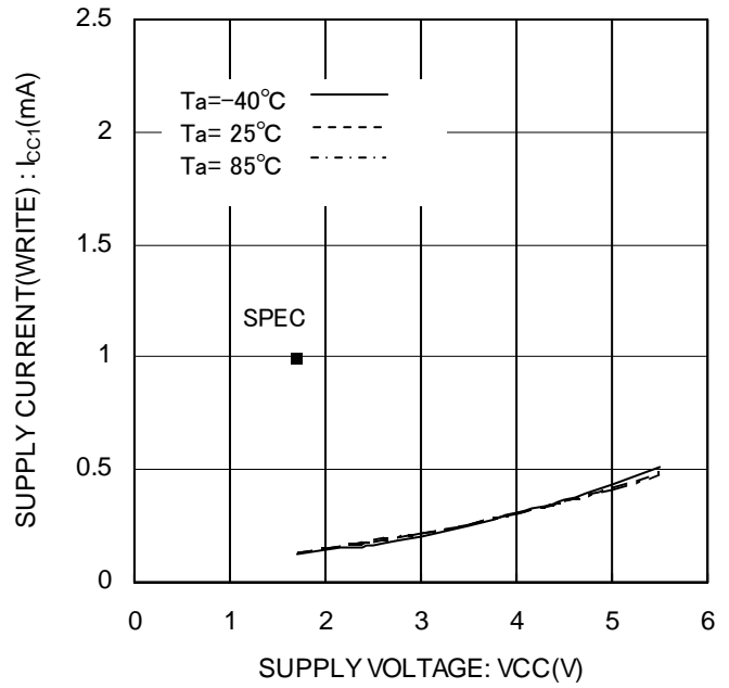
Figure 13. Supply current (WRITE) I_{CC1} (WRITE, f_{SK}=1\text{MHz} )
