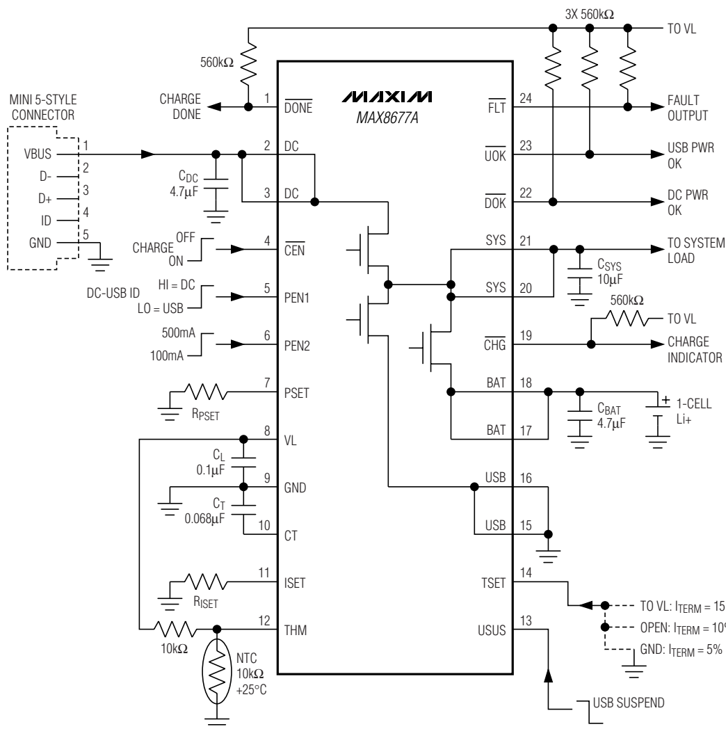
Figure 3. Typical Application Circuit Using Mini 5-Style Connector or Other DC/USB Common Connector
