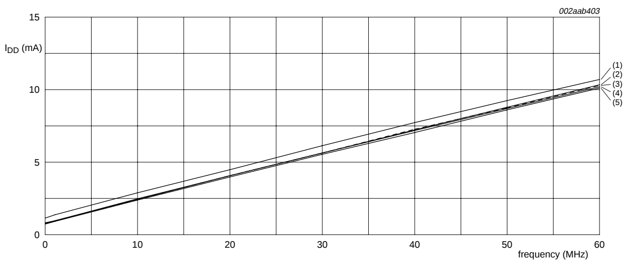
Fig 11. I_{DD} idle measured at different frequencies (CCLK) and temperatures
