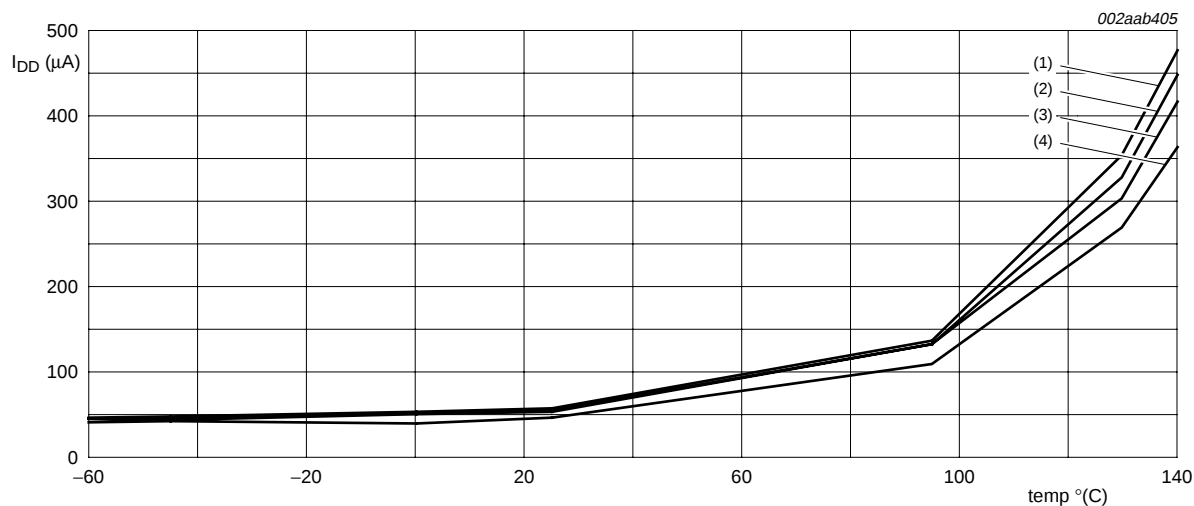
Fig 12. I_{DD(pd)} measured at different temperatures
