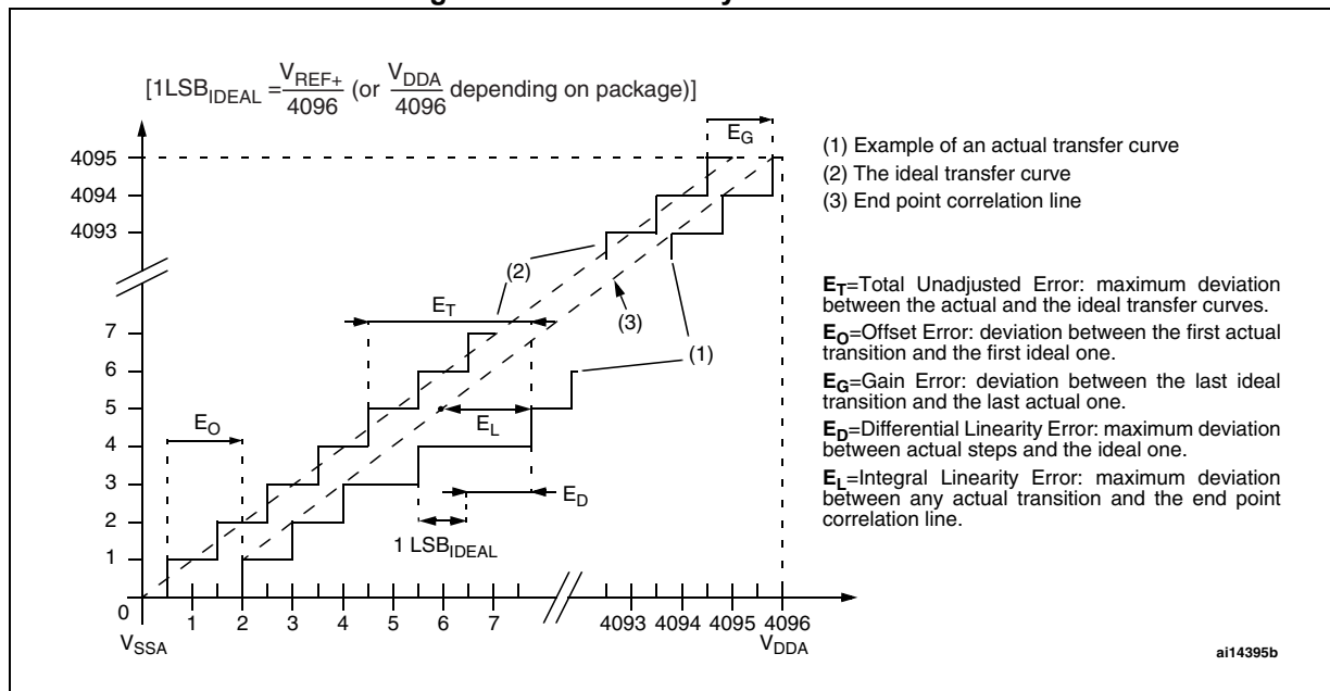
Figure 57.ADC accuracy characteristics
