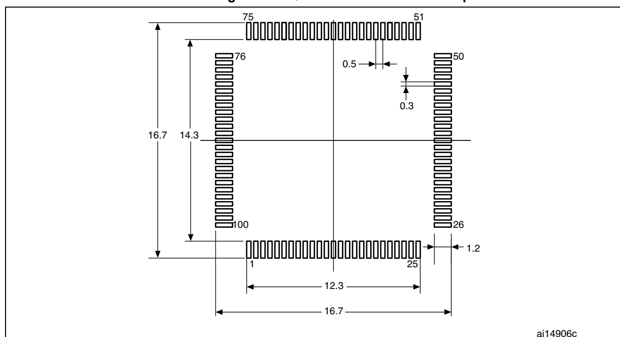
Figure 71.LQFP100 recommended footprint
