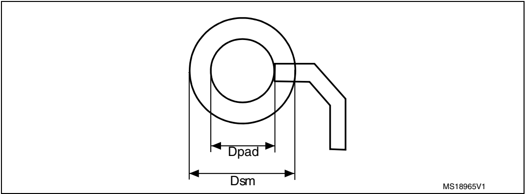
Figure 66.BGA pad footprint
