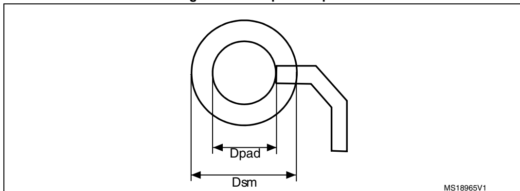
Figure 62.BGA pad footprint
